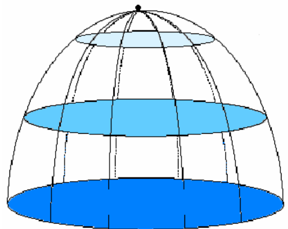
Standard spray sprinkler discharge pattern
